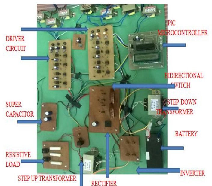
Fig 9. Hardware setup
