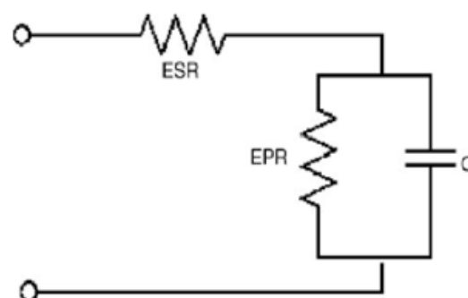
Fig3. Equivalent circuit of ultracapacitor[6]
