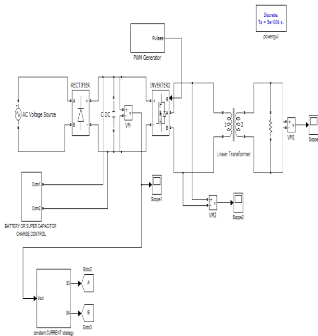
Fig 5. Simulation circuit of the modeled RAPS system
