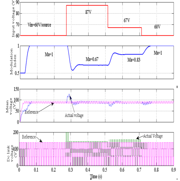
Fig. 8. Simulation results of control action on DC side for K_p=1.78 , K_i=0.72
