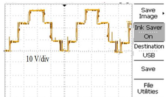
Fig. 10. Voltage level in switching devices for different switching time period
