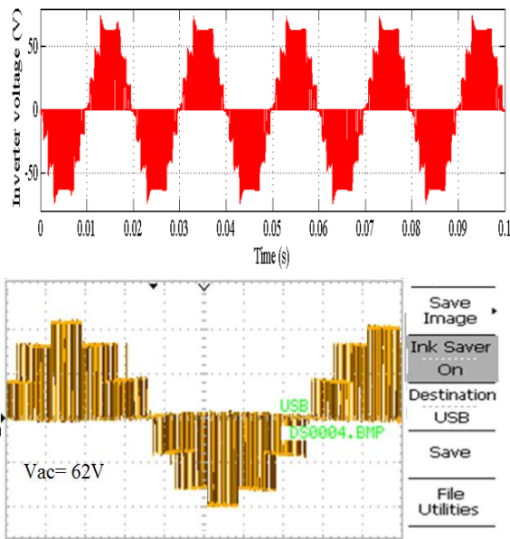
Fig. 11. Prototype photo, Simulation and hardware output of RSqZMLI for input voltage of B_1=24V , B_2=12V . \alpha=22\%
