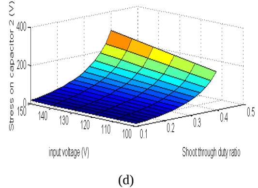
Fig. 6. Analysis of RSqZMLI for different shootthrough duty ratio
