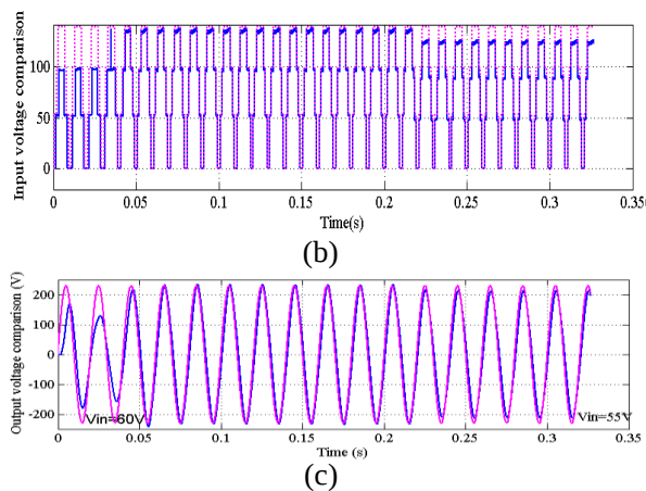
Fig. 9. Simulation results of control action on inverter side for K_p=1.78 , K_i=0.72
