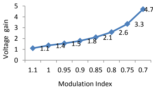
Fig. 2. Voltage gain of RSqZMLI for different M_a
