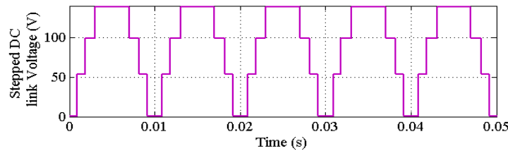
Fig. 5. Simulation result of stepped DC voltage ( V_{sdc} )
