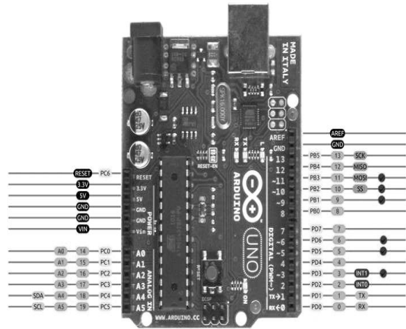
AVR DIGITAL ANALOG POWER SERIAL SPI I2C PWM INTERRUPT
