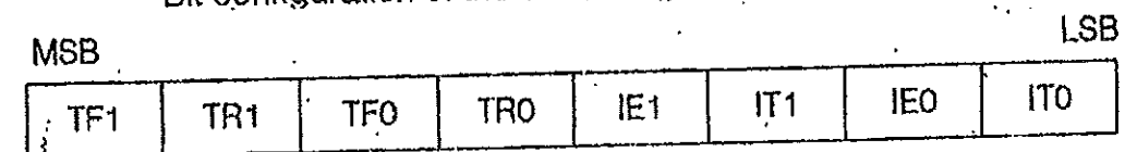
TCON bits used for timer programming
