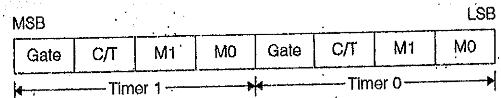
Bit configuration of the TMOD register
