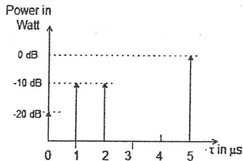
Figure 1: Power delay profile
